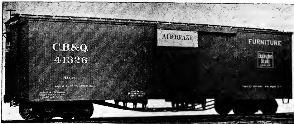
Fig. 4. FURNITURE CAR. CHICAGO, BURLINGTON & QUINCY RAILROAD. Length, 40 ft. Capacity, 50,000 lbs. Weight, 31,850 lbs. Coupler is placed between Center Sills to get greater height of Car-body. (Details are shown in Figs. 247-250.)
